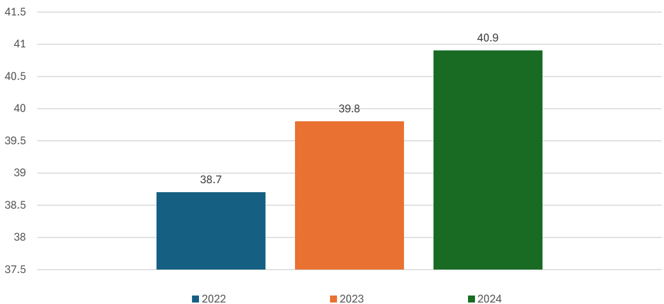
Attainment 8 score
